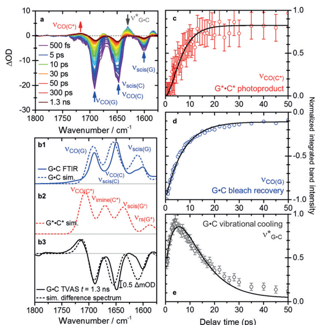
Figure 3. Transient vibrational absorption spectra, calculated vibrational spectra, and time profiles after excitation of G·C at 260 nm. a) Transient IR spectra of G·C in CDCl 3 . b1, b2) Experimental (solid lines) and calculated IR (dashed lines) spectra for the G·C WC structure and the G*·C* tautomer. b3) Difference spectra of G*·C* and G·C (simulated assuming \Phi = 7\% ) compared with the experimental transient spectrum at 1.3 ns. c–e) Time profiles (○) and fit results (—) to the spectral features centered at 1720 cm -1 (c), 1693 cm -1 (d), and 1630 cm -1 (e). Labels indicate the vibrational character of bands (see Table S2). The transient spectra were smoothed using a running average with one neighboring pixel. Calculations were performed at the B3LYP/6-311 + G** level of theory.
